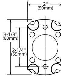
Snap Flange
